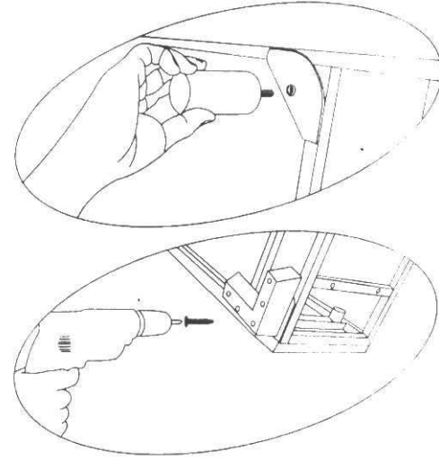
L LEGS SET-UP DIAGRAM
