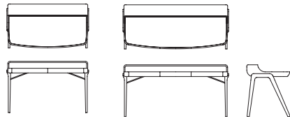
PICARD working desk / Arbeitstisch 120x60x88 cm 143x75x88 cm 183x75x88 cm SOLID WOOD TOP / CORIAN TOP / PAINTED TOP
