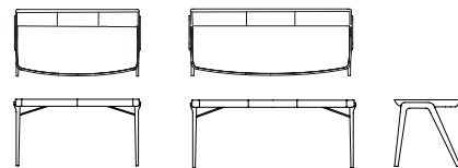
PICARD working desk / Arbeitstisch 120x60x76 cm 143x75x76 cm 183x75x76 cm SOLID WOOD TOP / CORIAN TOP / PAINTED TOP
