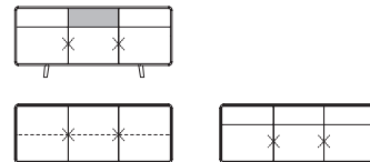
NEVA sideboard / Anrichte H 90 W 200 D 47 CM 3 DOORS + 3 DRAWERS / 3 DOORS / 3 DOORS + 2 DRAWERS + 1 OPEN PART
