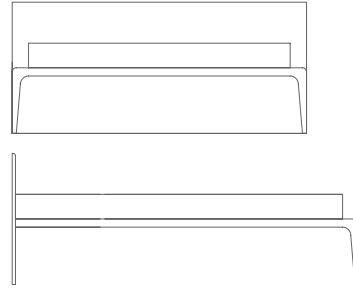
W 90, 140, 160, 180, 200 D 200 CM WITHOUT DRAWERS AND WITH REGULAR HEADBOARD
